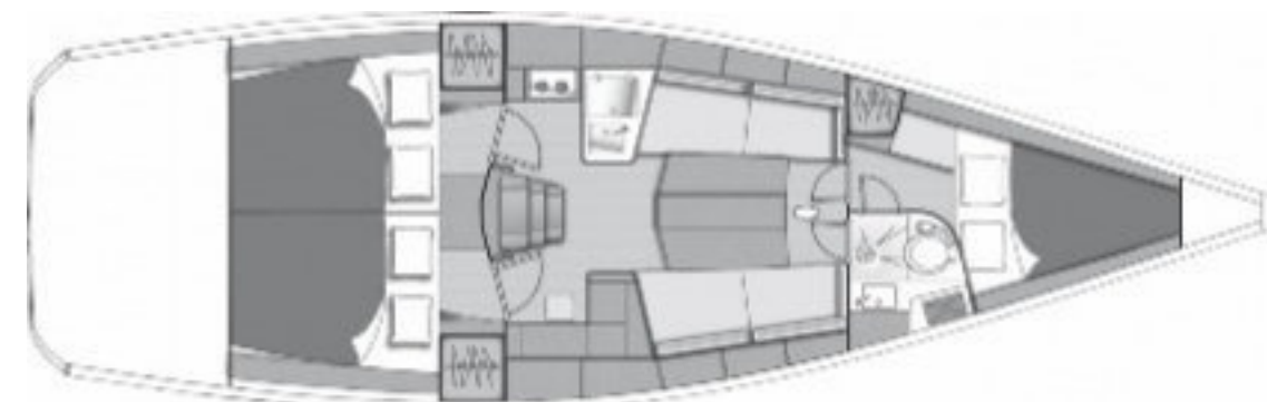
BENETEAU FIRST 40 INSIDE LAYOUT
